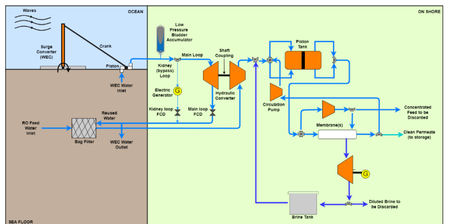
Figure 1: Prototype PRO-BRO schematic combined with the improved WEC design.
